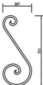
PART # SSU / 08
