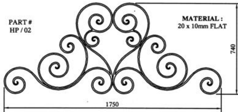
HEAD PIECE - 02
