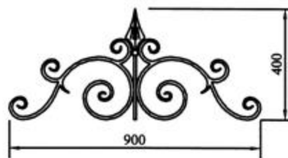
HEAD PIECE - 03
