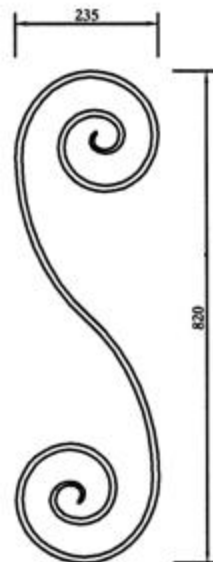
PART # SS / 10
