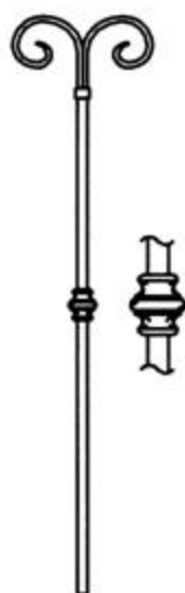
EIW 205 □16mm SCROLLS : 16 x 8mm FERRULE CAST 900 H x 216 W HEB / PL
