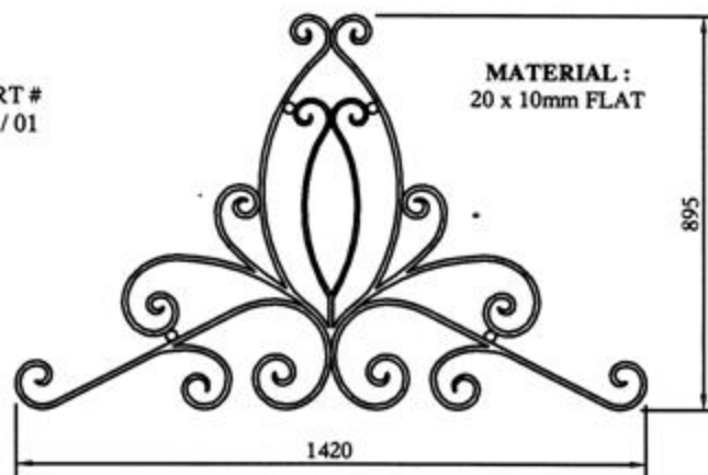
CENTER PIECE - 01
