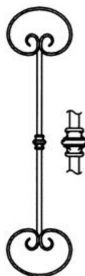
EIW 203 □16mm SCROLL : 16 x 8mm FERRULE CAST 900 H x 216 W HEB / PL
