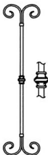
EIW 207 □16mm SCROLLS : 16 x 8mm FERRULE CAST 900 H x 216 W HEB / PL
