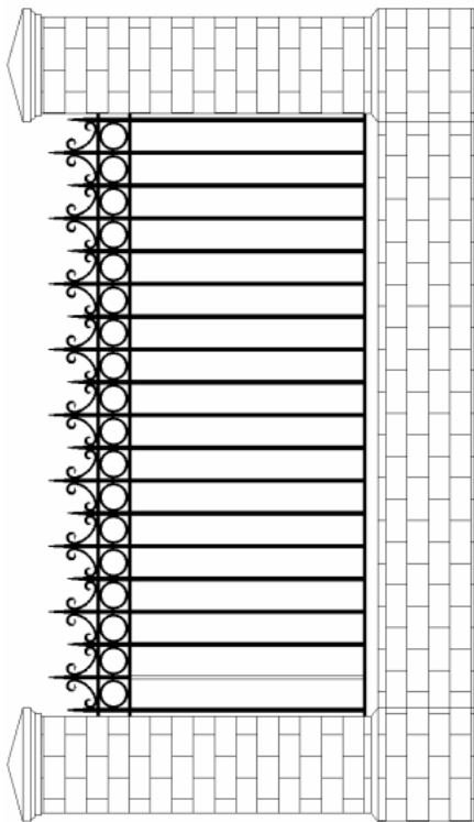
FENCE PANEL - 09
