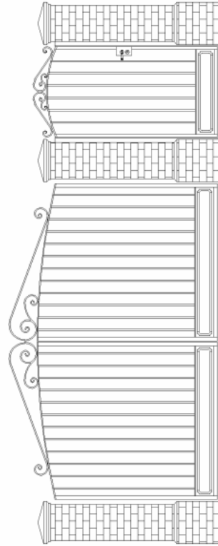
GATE DESIGN G-16
